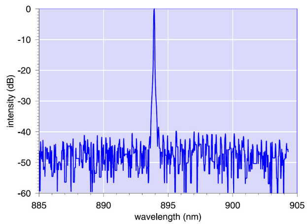
Room Temperature CW Spectrum at 894nm
